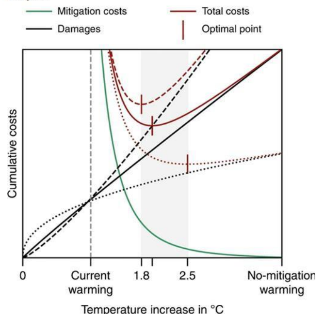
Fig. 1: Illustration of universality of the cost-benefit climate analysis.
